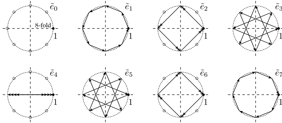
Figure 7. The Fourier base vectors \tilde{e}_k of \mathbf{C}^8 , 0 \leq k \leq 7 , are the regular \{8/k\} -gons \left( (e^{i2\pi/8})^{k \cdot 0}, (e^{i2\pi/8})^{k \cdot 1}, \dots, (e^{i2\pi/8})^{k \cdot 7} \right) .
